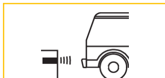
Object Detection
