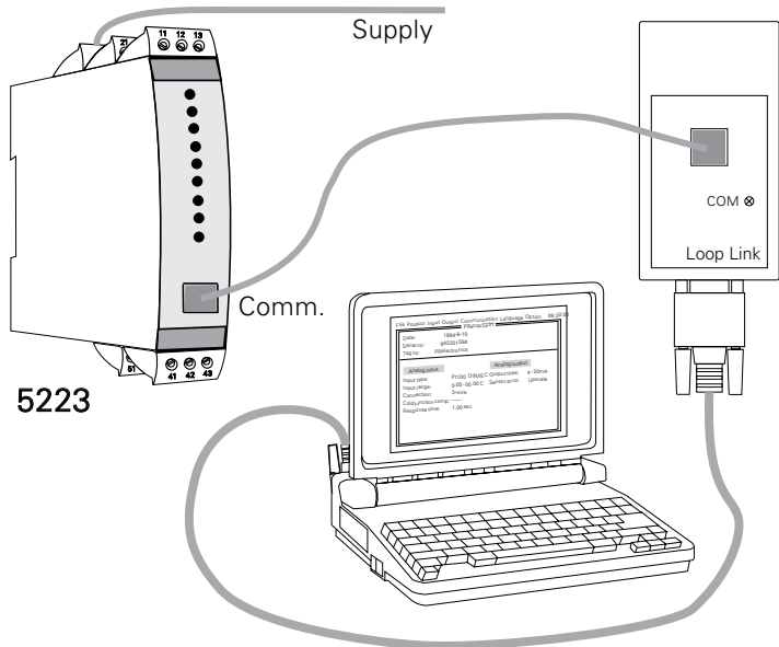
5223 connection to Loop Link:
