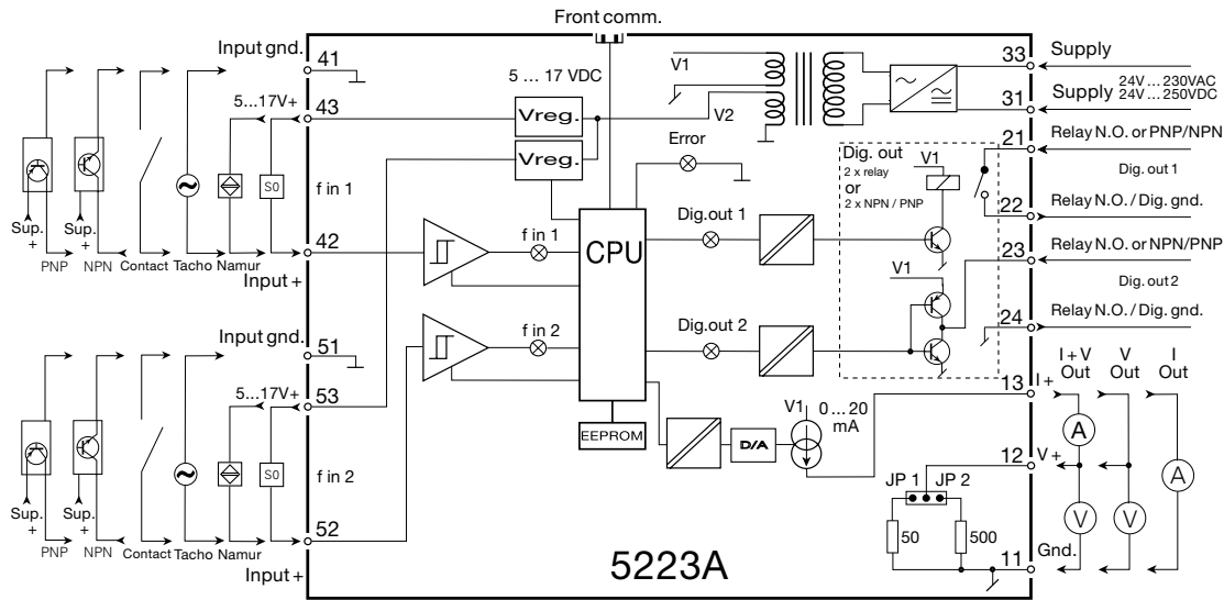
Block diagram, 5223B:
