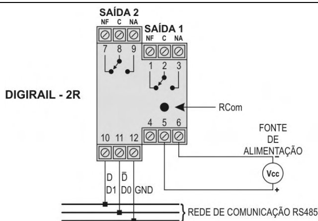
Figure 2 – Electrical Connections
