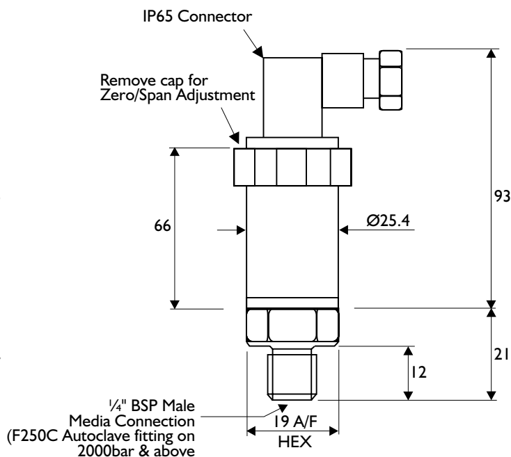
Dimensions for 2 to 2500 bar ranges
