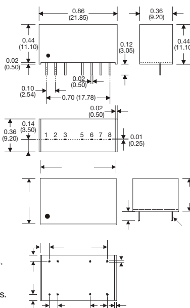
All dimensions in inches (mm).
